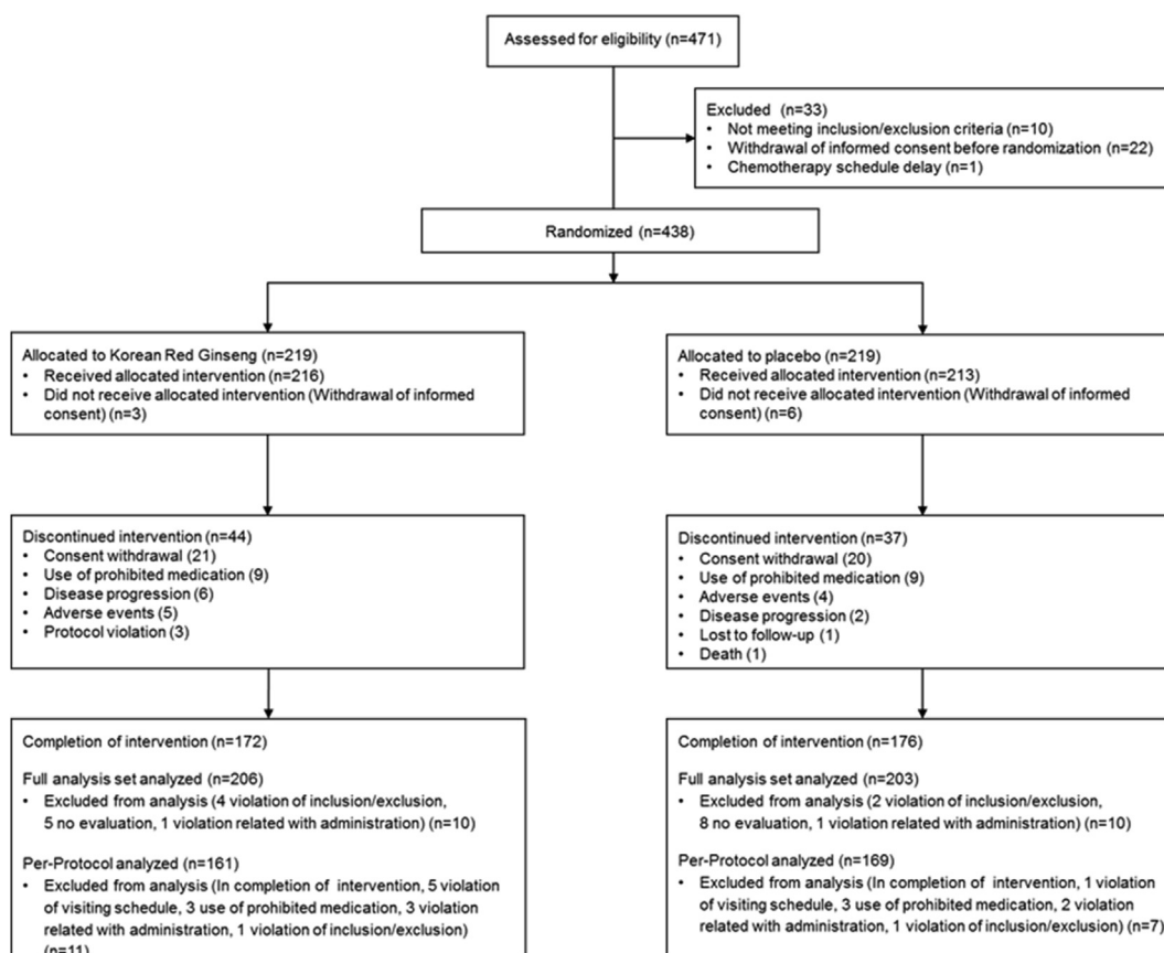
Fig. 1. CONSORT diagram.
